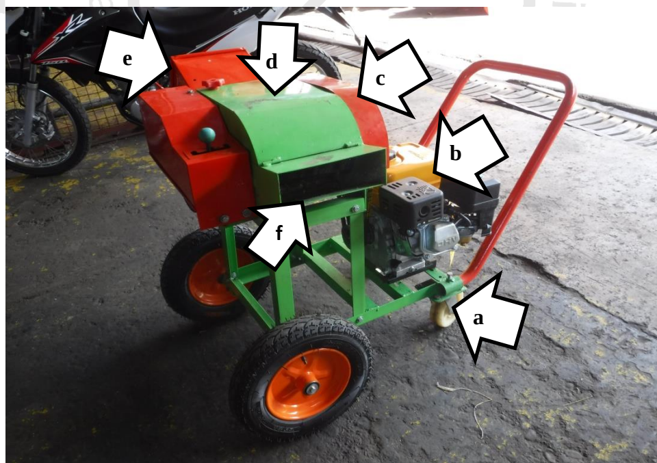
Figure 1. Parts of Forage Chopper CIAMC 9 ZP-0.4 powered 4.8 kW TOYOHAMA TH168F2 Gasoline Engine include the following: (a) Transport wheels, (b) Prime mover, (c) Belt-pulley transmission system, (d) Cutter assembly, (e) Input chute, and (f) Discharge chute.
